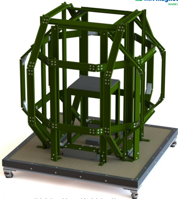
A custom 3-axis Helmholtz coil designed for CubeSat calibration.
